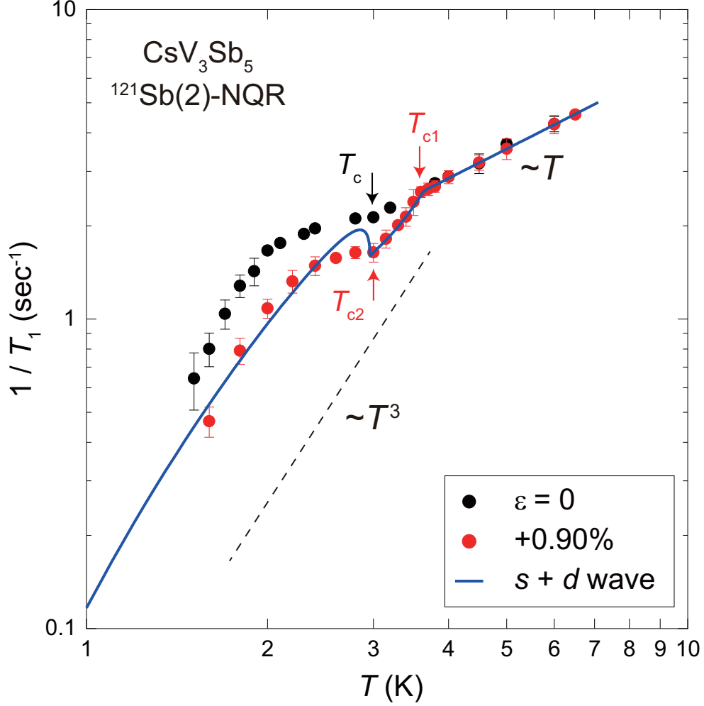
FIG. 4. Temperature dependence of the ^{121}\text{Sb}(2)\text{-NQR} 1/T_1 at \varepsilon = 0 and +0.90\% . Arrows indicate the respective superconducting transition temperatures, T_c . The solid and dashed lines show linear ( \sim T ) and cubic ( \sim T^3 ) dependencies above and below T_c , respectively, as guides to the eye. The solid curve represents the fitting result with a two-component ( s + d wave) model (see text). Error bars represent the standard deviations from the fitting parameters.
