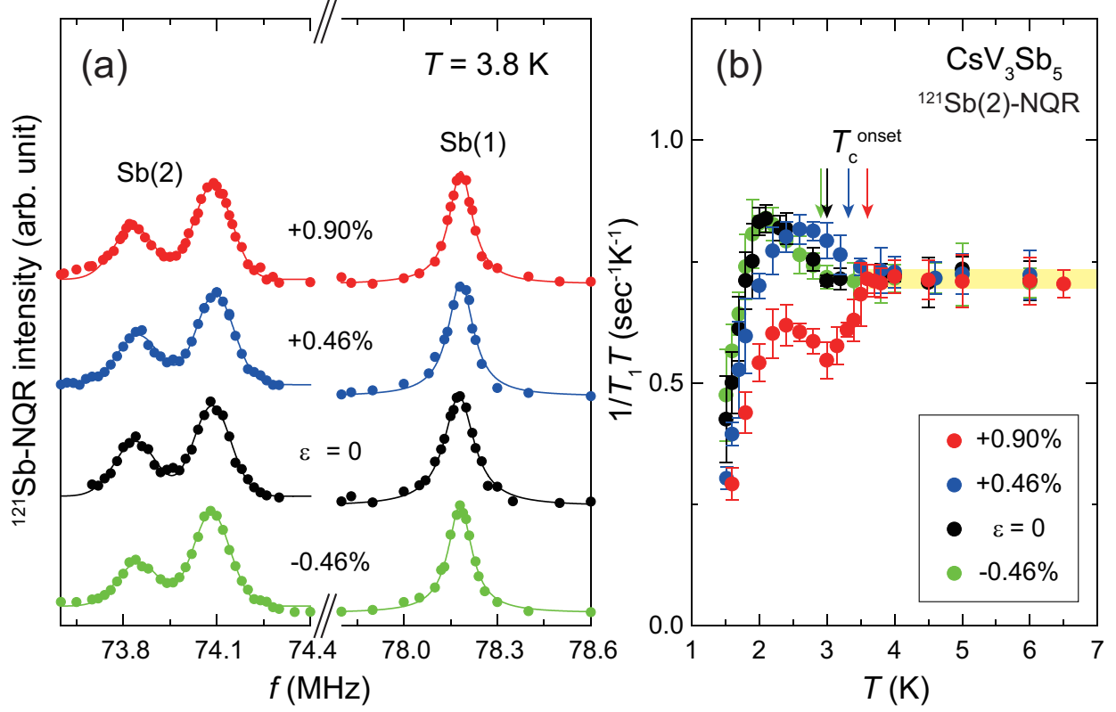
FIG. 2. (a) Strain dependence of the ^{121}\text{Sb} -NQR spectra in the CDW state at T = 3.8 K. The spectra consist of the Sb(2) lines (left, \sim 74 MHz) and the Sb(1) line (right, \sim 78.2 MHz). The solid curves represent the best fits using a sum of two Gaussian functions for the Sb(2) site and a single Lorentzian function for the Sb(1) site. (b) Temperature dependence of the ^{121}\text{Sb} -NQR 1/T_1T for various strains, measured at the Sb(2) site ( f = 74.1 MHz). The horizontal line is a guide to the eye. Error bars represent the standard deviations from the fitting parameters.
