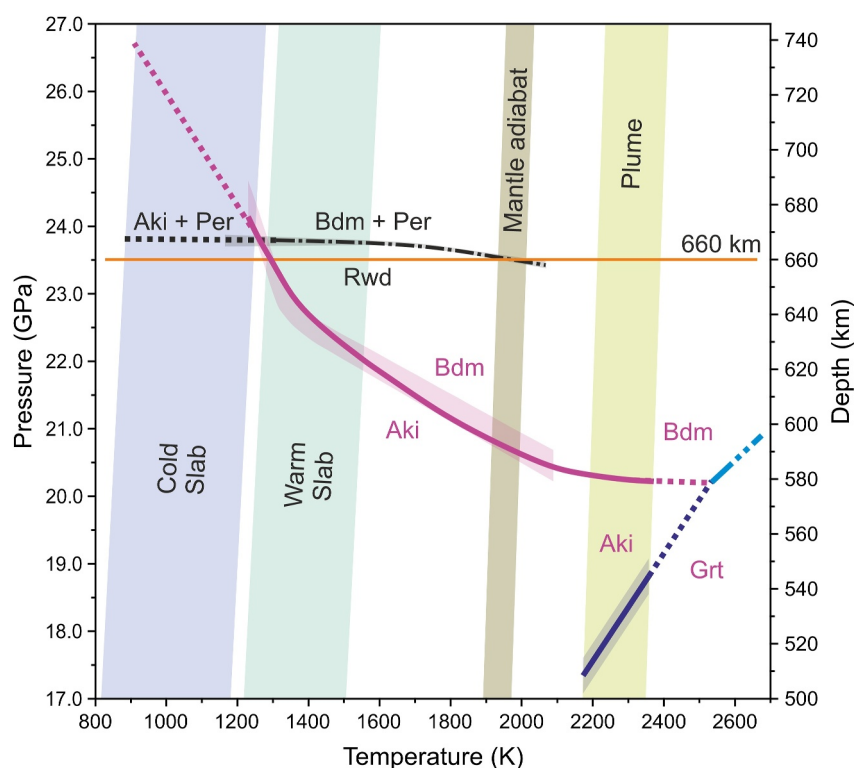
Figure 4. Combination of the present results with previous data from (Chanyshv et al., 2022) in MgO-SiO 2 systems. Cold and warm subduction geotherms are from (Ganguly et al., 2009; Thompson, 1992), and the average mantle geotherm is from (Katsura, 2022). The plume geotherm is drawn assuming that the temperatures in plumes are 200–300 K higher than the ambient mantle (Karato, 1993; Katsura, 2022; White & McKenzie, 1995). The horizontal solid orange line indicates 660 km depth (Dziewonski & Anderson, 1981). The Rwd dissociation boundary from (Chanyshv et al., 2022) is shown as a dot-dashed black curve and gray-shaded area. The Aki-Bdm transition boundary is shown by a solid violet curve. The Grt-Aki boundary is shown as solid dark blue curve and blue-shaded area. The dotted lines are the result of linear extrapolation of the Rwd dissociation boundary below 1,300 K, the Aki-Bdm boundary below 1,300 K and above 2,350 K, and the Aki-Grt boundary above 2,350 K. The dash double dotted blue line is the calculated Grt-Bdm boundary based on the slopes of Aki-Bdm and Grt-Aki boundaries at temperatures above 2,200 K. Aki, MgSiO 3 akimotoite; Bdm, MgSiO 3 bridgmanite; Per, MgO periclase; Rwd, Mg 2 SiO 4 ringwoodite; Grt, MgSiO 3 majorite garnet.
