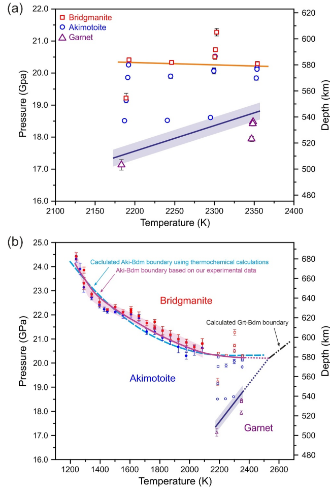
Figure 2. Phase relations in the MgSiO 3 system. (a) Aki-Bdm and Grt-Aki phase transition boundaries determined in the current study at 2,150–2,350 K and 17–21 GPa. (b) MgSiO 3 phase diagram at 1,200–2,600 K and 17–25 GPa. Red squares, blue circles, and purple triangles indicate the P–T conditions of Bdm, Aki, and Grt stability fields, respectively. Open and filled symbols are from the current study and from Chanyshv et al. (2022), respectively. Pressures were determined from the MgO unit-cell volumes using the Birch–Murnaghan and Vinet equations of state from Tange et al. (2009). Error bars result from the pressure uncertainty of the MgO equation of state suggested by Tange et al. (2009). The temperatures and pressures were corrected based on the pressure effects on the thermoelectromotive force of a W 97 Re 3 –W 75 Re 25 thermocouple (Nishihara et al., 2020). The dark blue shaded area indicates an allowed region for the Aki-Bdm boundary. The solid dark blue line represents the most likely transition curve within this range. The orange line on top figure (a) indicates the Aki-Bdm phase transition boundary based on experimental data obtained in this study. The violet shaded area indicates an allowed region for the Aki-Bdm boundary for most experimental data points. The solid violet curve represents the most probable transition curve within this area. Dotted lines are result of linear extrapolation of the Aki-Bdm and Aki-Grt transition boundaries above 2,200 K. The dashed blue line indicates the Aki-Bdm phase transition boundary calculated from the proposed heat capacities difference (Figure S2 in Supporting Information S1). The dash dotted black curve is calculated Grt-Bdm boundary based on the slopes of Aki-Bdm and Grt-Aki boundaries at temperatures above 2,200 K.
