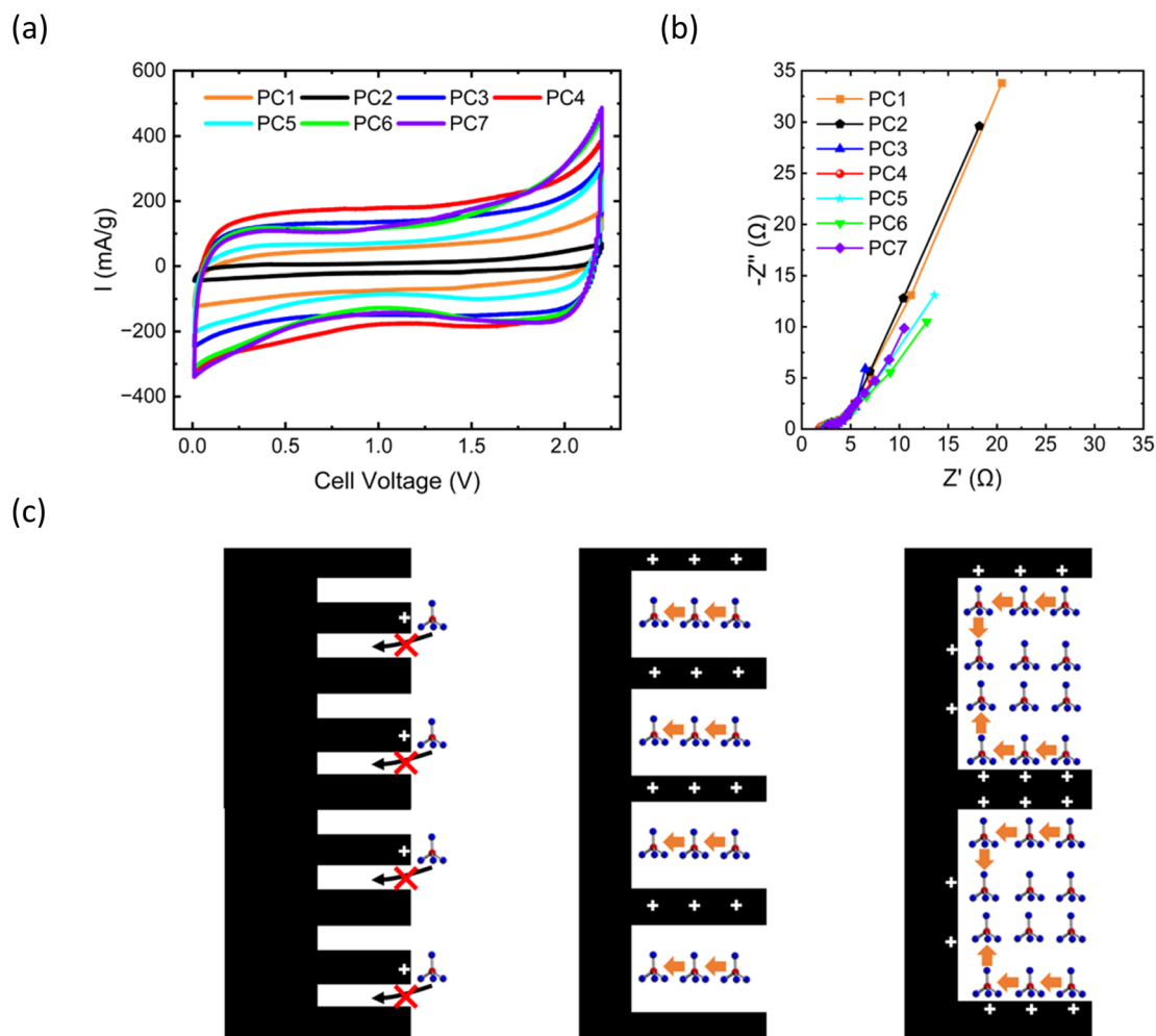
Fig. 4 Rechargeable porous carbon/aluminium cell. (a) Cyclic voltammetry of Al foil and PC at a scan rate of 1 \text{mV s}^{-1} . (b) Nyquist plots of PC1–7 at 2.2 V and at an amplitude of 10.0 mV and frequencies ranging from 1.0 MHz to 0.1 Hz. (c) Model diagram of the adsorption of \text{AlCl}_4^- ions on the PC cathodes. PC1 (YP50F), PC2 (MSP-20), PC3 (MSA-20), PC4 (MSC-30), PC5 (CNovel 20 nm), PC6 (CNovel MJ4 010-00), and PC7 (CNovel MH-00); PC, porous carbon.
