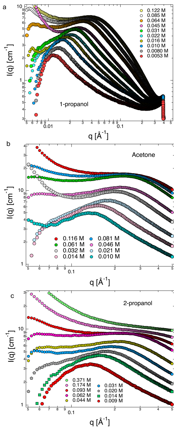
FIG. S2. SAXS profiles for TBAPSS in three low dielectric constant solvents at selected concentrations indicated on the legend.
