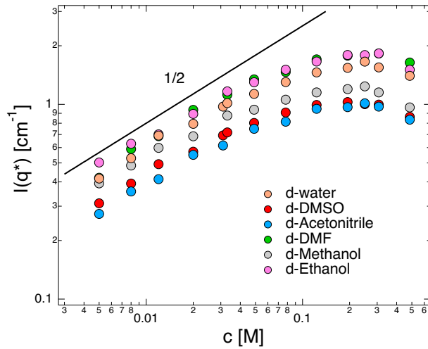
FIG. S1. SANS intensity at the peak position after subtraction of high- q plateau. Line is power-law exponent of I(q^*) \propto c^{1/2} .
