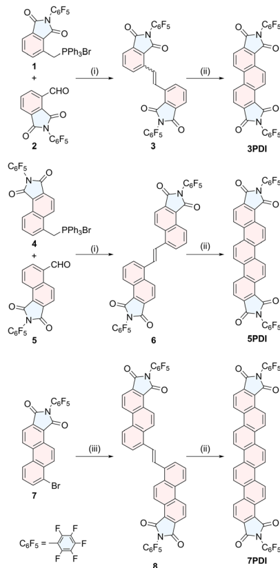
Scheme 1 Synthetic routes to n PDI. Reagents and conditions: (i) Bu 4 NF, CH 2 Cl 2 , (ii) hν , I 2 , air, toluene, (iii) K 2 CO 3 , Bu 4 NBr, CH 2 Cl 2 -THF then Bu 4 NF, (iv) ( E )-1,2-bis(tetrabutylstannyl)ethene, Pd(PPh 3 ) 4 .
