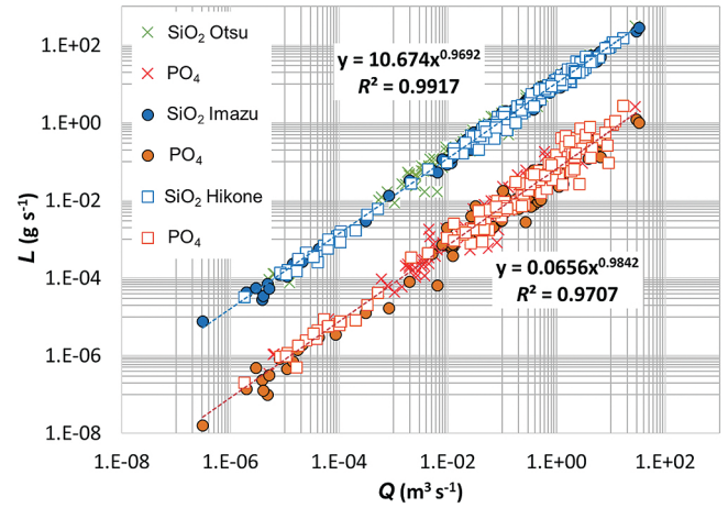
Figure 4. The loading curve for \text{PO}_4 and \text{SiO}_2 which were regarded as unified for these nutrients. The correlation coefficients between L and Q were R^2 = 0.99 ( \text{SiO}_2 ) and R^2 = 0.97 ( \text{PO}_4 )
