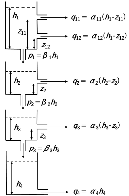
Figure 2. Structure of the tank model. The surface discharge ( q_{11} + q_{12} ), intermediate discharge ( q_2 ), sub-base discharge ( q_3 ), and base discharge ( q_4 ), p is infiltration to the lower reservoir, \alpha and \beta are the coefficients, h is the water level, z is the outlet height
