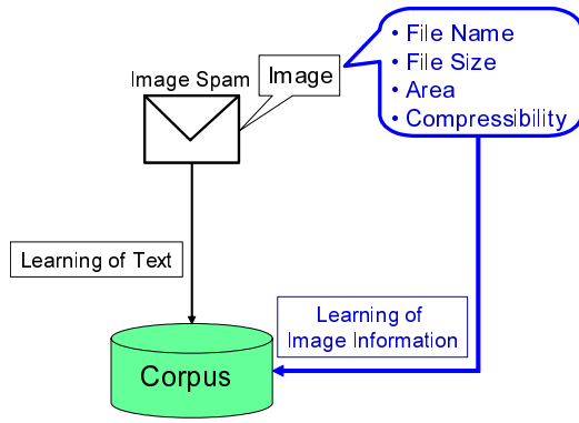
Figure 5. Learning flow
