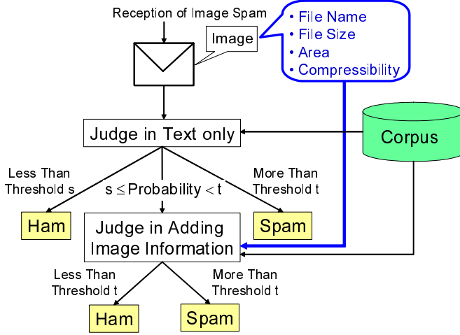
Figure 6. Judgment flow
