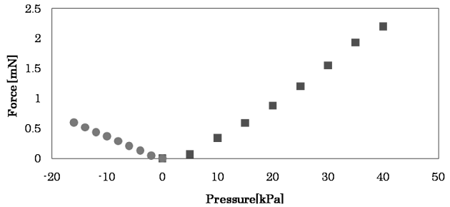
Figure 21. Experimental results of force measurement.
