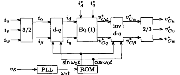
Fig. 3. Control circuit of the series device.
