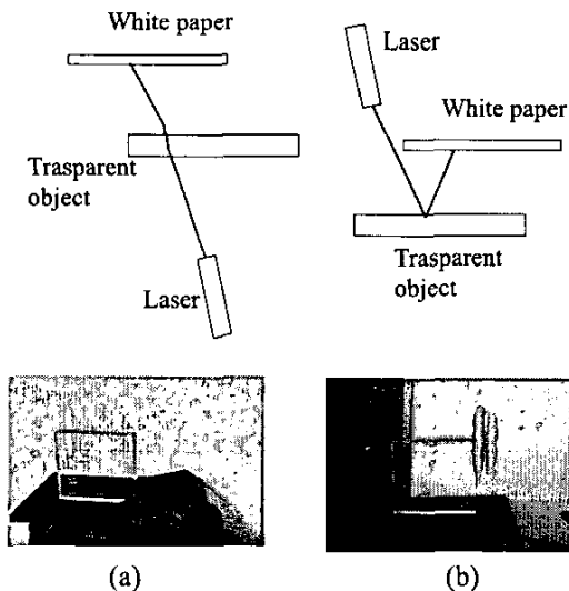
Fig. 5 Observed results when a light-stripe was projected onto a transparent acrylic plate.
