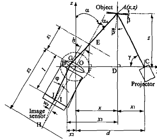
Fig.4 Coordinate system
