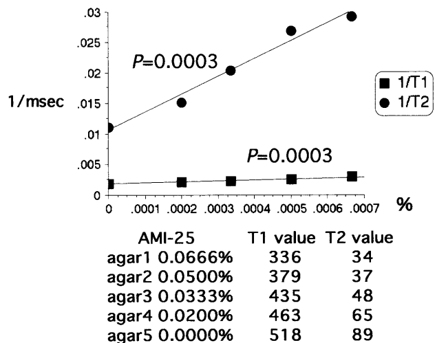
Fig. 1 The correlation between 1/\text{T1} or 1/\text{T2} and the concentration of SPIO. A strong correlation is seen between 1/\text{T1} or 1/\text{T2} and the concentration of SPIO.
