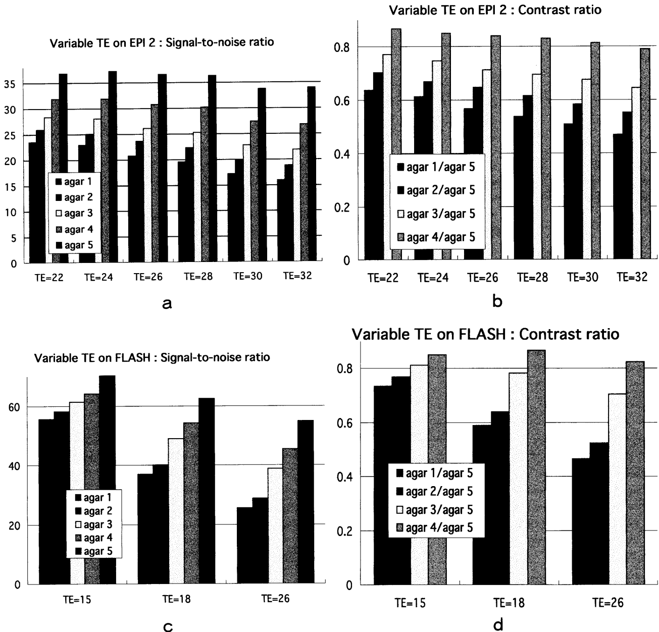
Fig. 4 Relationships between S/N, CR, and effective TE for each GRE sequence.
