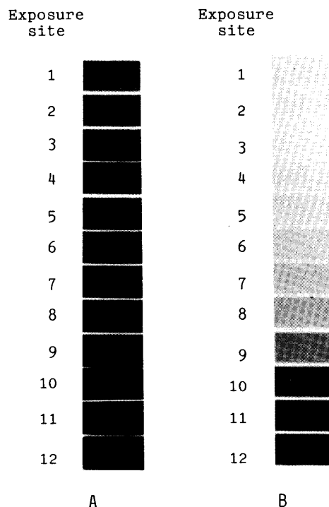
Fig. 1 Film strips exposed according to the modified inverse square sensitometric method (EM/RX screen/film system). A: First series of exposures in which the x-ray beam was filtered through the basic filter. B: Second series of exposures in which the x-ray beam was filtered through a 1.1 mm copper filter in addition to the basic filter.
