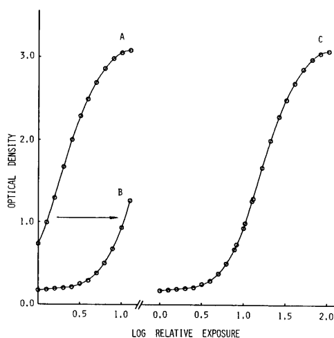
Fig. 2 Characteristic curve drawn by modified inverse square sensitometry (EM/RX screen/film system). A : The segment of the characteristic curve obtained in the 1st exposure series. B : The segment of the characteristic curve obtained in the 2nd exposure series. C : The entire characteristic curve obtained by shifting A to overlap B.
