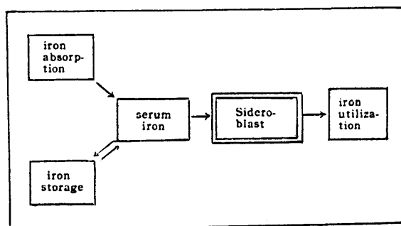
Fig. 6. Diagrammatic Description of Iron Movement in Relation to Sideroblasts
