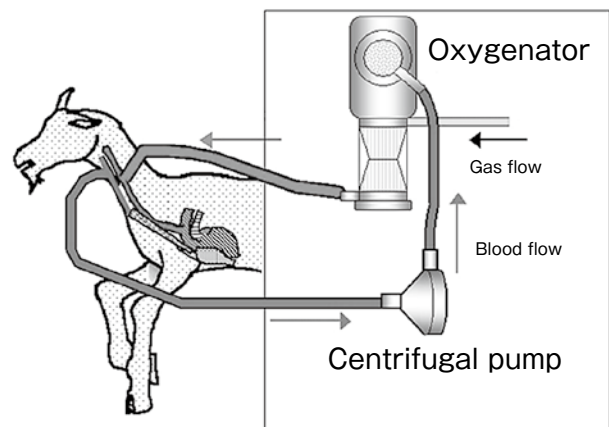
Fig. 1 Schematic illustration of the experimental percutaneous cardiopulmonary support circuit (Capiex EBS, Terumo Corporation, Kanagawa, Japan). The circuit was placed between the superior vena cava via the right jugular vein for withdrawal and right carotid artery for supply.
