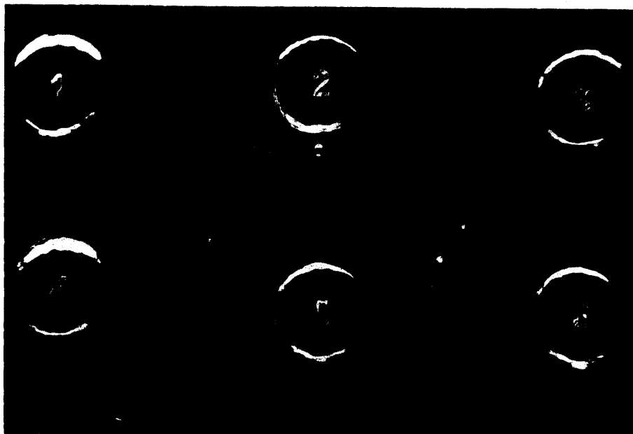
Fig. 5. Immuno-electrosyneresis with positive precipitin reactions in sera of systemic lupus erythematosus (well No. 4 and 5), against membrane solution after reducing SDS to the level of 10^{-6}M (well No. 1, 2 and 3). The serum of a healthy individual (well No. 6) showed no reaction. The anode is on the upper side.
