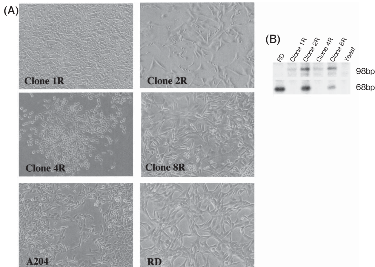
Fig. 7 Stable transfection with a GFP-linked COL3A1 promoter. (A) Stably transfected cells. Clones 1R, 2R, 4R and 8R were derived from RD cells. Note that the cell shapes of clones 1R and 4R are similar to that of A204 cells, but not to that of RD cells. (B) RNase protection assay using stably transfected cells. Data from clones 1R, 2R, 4R and 8R are shown.
