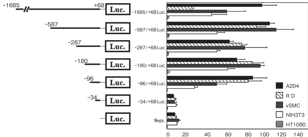
Fig. 2 Luciferase transcription activity of the COL3A1 promoter using the 5'-deletion reporter constructs. Luciferase activities in A204, RD, vSMC, NIH3T3 and HT1080 cells were measured. The data for A204 cells have been previously published [12]. All the constructs were cotransfected with the pRL-SV40 vector as an internal control for transfection efficiency. Relative luciferase activities (%) were normalized to the activity of the -1685 to +68 Luc construct and transfected into A204 cells. Data are the means \pm SD values of at least 3 independent experiments.
