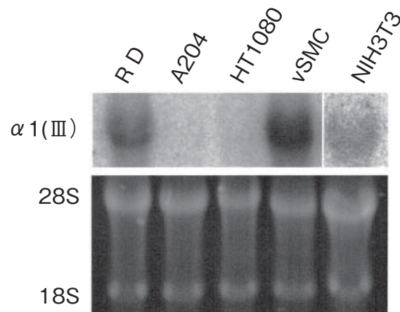
Fig. 1 Northern blot analysis to show COL3A1 RNA expression in various cell types. Upper panel: RNAs were hybridized with an \alpha 1(\text{III}) cDNA probe. Lower panel: the gel was stained with ethidium bromide to identify the locations of 28S and 18S rRNA. RD, human embryonal rhabdomyosarcoma cell line; A204, human rhabdomyosarcoma cell line; HT108, human fibrosarcoma cell line; vSMC, bovine vascular smooth muscle cell.
