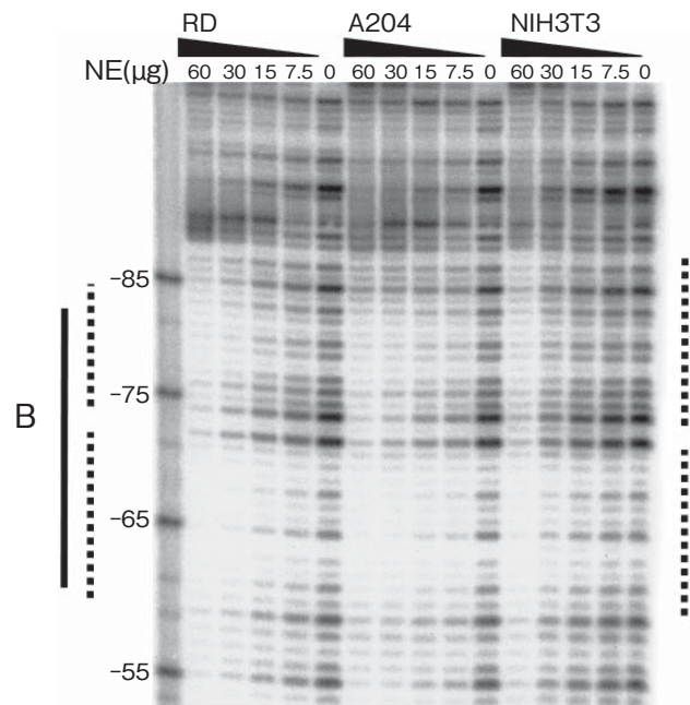
Fig. 5 DNase I footprinting analysis of the region around the B element of the COL3A1 promoter. The [ 32 P]-labeled –97 to –31 probe was incubated with RD, A204 and NIH3T3 nuclear extracts. B: B element. Dotted lines indicate protected regions.
