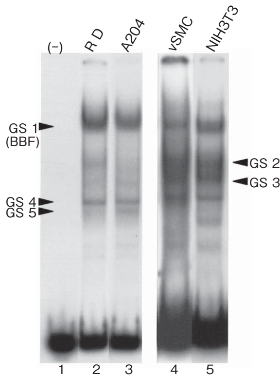
Fig. 4 EMSA analysis of the COL3A1 promoter. The [ 32 P]-labeled –97 to –31 probe was incubated with nuclear extracts from RD, A204, vSMC and NIH3T3 cells. The DNA-protein complexes are the GS1(BBF), GS2, GS3, GS4 and GS5 bands, which are indicated by arrowheads. Lane 1 contains no nuclear extract. Extra bands were sometimes seen depending on the preparation of the nuclear extracts.
