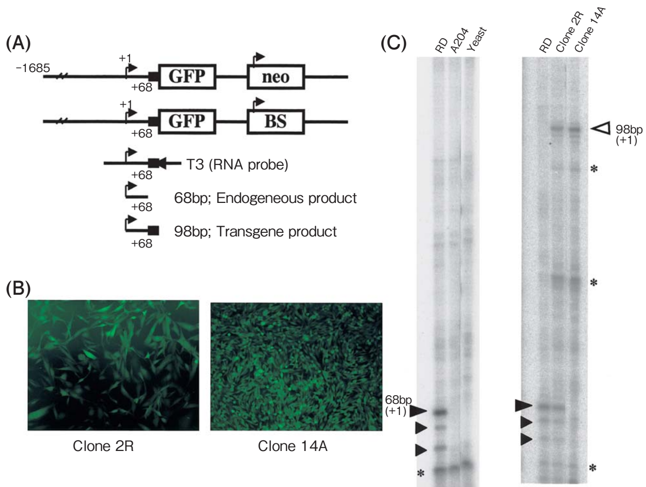
Fig. 6 Stable transfection with a GFP-linked COL3A1 promoter. (A) Schematic illustration of constructs of the GFP-linked COL3A1 promoter, the RNA probe, and gene products. (B) Stably transfected cells. Note that clone 2R and clone 14A derived from RD and A204 cell lines, respectively, show expression of type III collagen. (C) RNase protection assay using stably transfected cells. Large and small closed triangles, an open triangle, and asterisks indicate major and minor endogenous gene products, the transgenic products, and nonspecific bands. Note that 2 minor transcripts from the endogenous gene were seen in the RD cells and in clone 2R.
