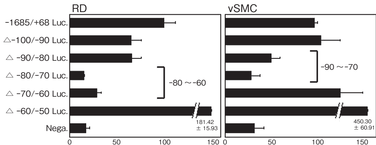
Fig. 3 Luciferase transcription activity of the COL3A1 promoter in RD and vSMC cells using the internal deletion constructs. All the constructs were cotransfected with the pRL-SV40 vector as an internal control for transfection efficiency. Relative luciferase activities (%) were normalized against the activity of the -1685 to +68 Luc construct transfected into each cell. Data are the means \pm SD values of at least 3 independent experiments.
