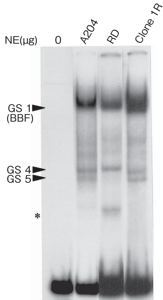
Fig. 8 EMSA analysis using nuclear extracts from A204 cells, RD cells and clone 1R. The [ ^{32} P]-labeled -97 to -31 probe was incubated with nuclear extracts from A204 cells, RD cells, or clone 1R cells. The DNA-protein complexes are the GS1 (BBF), GS4 and GS5 bands indicated by arrowheads. An asterisk indicates a nonspecific band. Lane 1 contains no nuclear extract.
