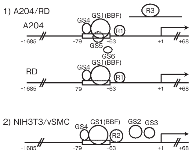
Fig. 9 Schematic summary of proteins binding to DNA in the proximal promoter region of the COL3A1 gene. The overview includes data from a previous study [12] and from the present study. R1, R2 and R3 are hypothetical repressors.
