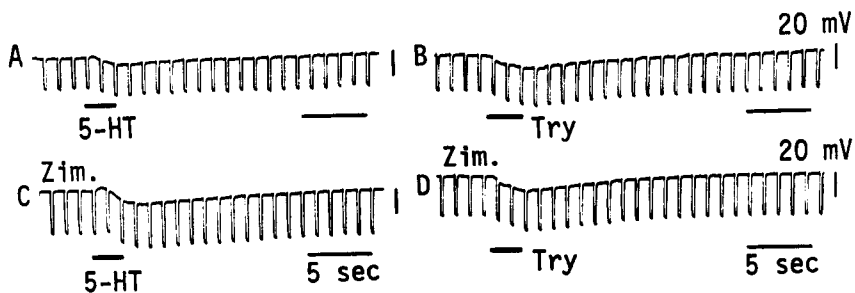
Fig. 3 No effect of superfusion with zimelidine (Zim; 10\mu\text{M} ) on the tryptamine (Try)-induced slow hyperpolarization in comparison with that on the 5-hydroxytryptamine (5-HT)-induced slow hyperpolarization in the same cell. The cell was injected with constant hyperpolarizing current pulses. A, Microinjection of 5-HT (short horizontal bar; two 999-msec pulses) evoked a slow hyperpolarization not associated with changes in input resistance. B, Microinjection of tryptamine (short horizontal bar; two 999-msec pulses) evoked a slow hyperpolarization without changes of input resistance. C, The slow hyperpolarizing response to 5-HT was not attenuated 7 min after beginning superfusion with zimelidine. D, The slow hyperpolarizing response to tryptamine was not attenuated 4 min after beginning superfusion with zimelidine. In C and D, zimelidine increased the amplitude of the electrotonic potentials. The resting membrane potential was -50\text{mV} .
