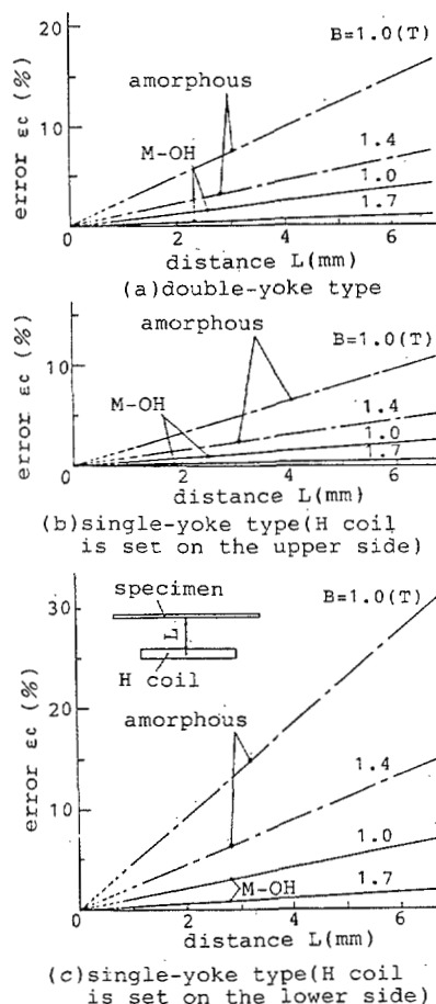
Fig. 6. Effects of H coil position for various constructions.
