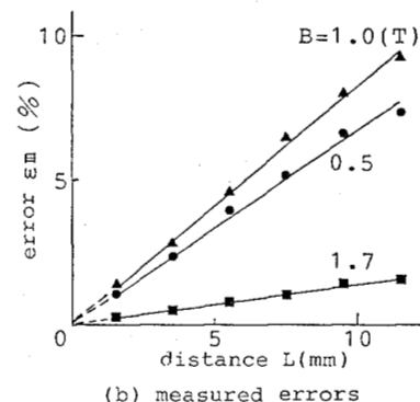
Fig.10. Effects of H coil position for highly oriented specimen.
