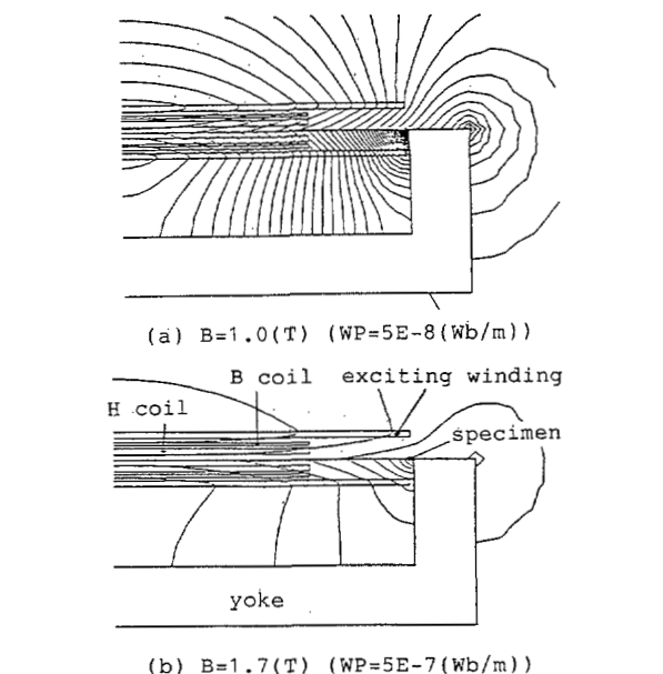
Fig. 4. Flux distributions for highly oriented specimen in the single-yoke type tester.
