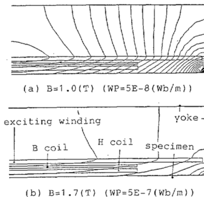
Fig.2. Flux distributions for highly oriented specimen in the double-yoke type tester.
