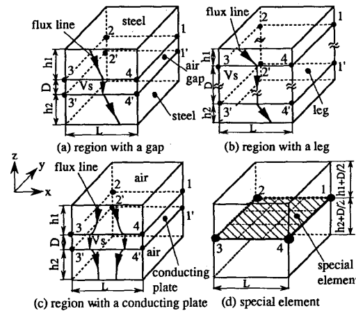
Fig. 1 Idea of various 3-D special elements.
