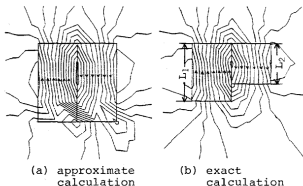
Fig. 13 Flux distributions.
