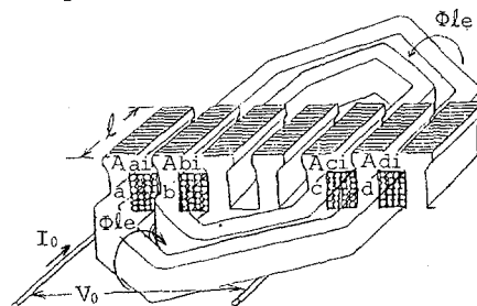
Fig. 3 Skeleton diagram.
