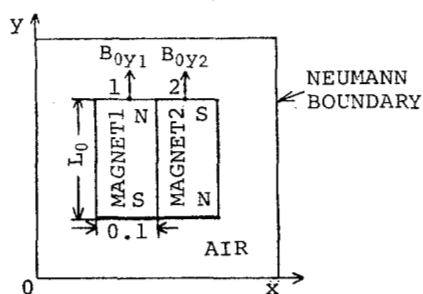
Fig. 12 Magnet model.
