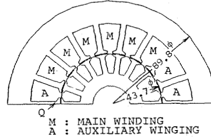
Fig. 9 Capacitor motor.
