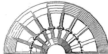
Fig.10 Flux distribution.
