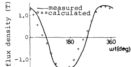
Fig. 11 Flux density waveform.
