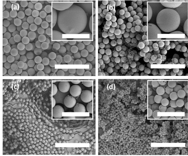
Fig. 3 SEM images of PLA microspheres prepared by solvent diffusion. The Q_c was (a) 600, (b) 1200, (c) 3,000, (d) 6,000 \mu\text{L h}^{-1} at a fixed Q_d (60 \mu\text{L h}^{-1} ). The concentrations of PLA and w-PEG-PLA were 1 wt%. The obtained microspheres were freeze-dried before SEM observation. Scale bars represent 100 \mu\text{m} . The inset is magnified view with a scale bar corresponding 20 \mu\text{m} .
