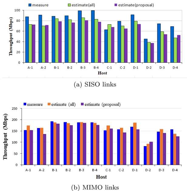
Figure 3: Measured and estimated throughput for AP5 in field#2.
