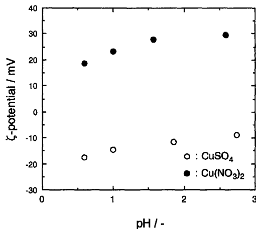
Fig. 5. Relation between \zeta -potential of \alpha - \text{Al}_2\text{O}_3 particle and solution pH for 0.5M \text{CuSO}_4 and 0.5M \text{Cu}(\text{NO}_3)_2 .
