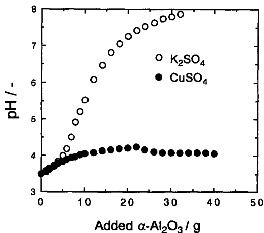
Fig. 6. pH shift for successive particle addition: 0.5M \text{CuSO}_4 , 0.5M \text{K}_2\text{SO}_4 initial pH = 3.5.
