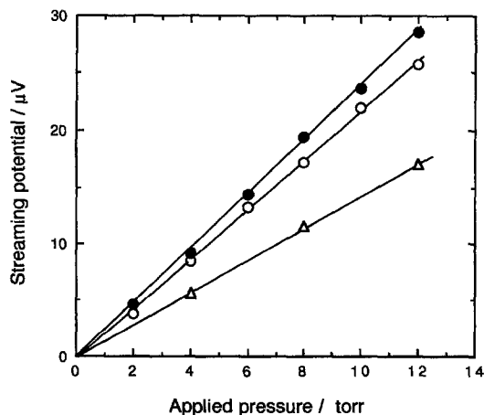
Fig. 4. The relationship between observed streaming potential and applied pressure for \alpha - \text{Al}_2\text{O}_3 particles in 0.5M \text{CuSO}_4 . ○: pH = 0.6, ●: pH = 1.0, △: pH = 2.7.
