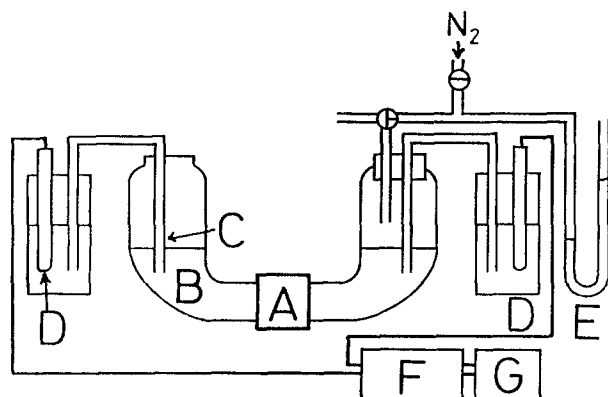
Fig. 1. Schematic diagram of streaming potential apparatus A: Plug B: Electrolyte solution C: Salt bridge D: Ag/AgCl electrode E: Hg manometer F: Microvolt meter G: Pen recorder.
