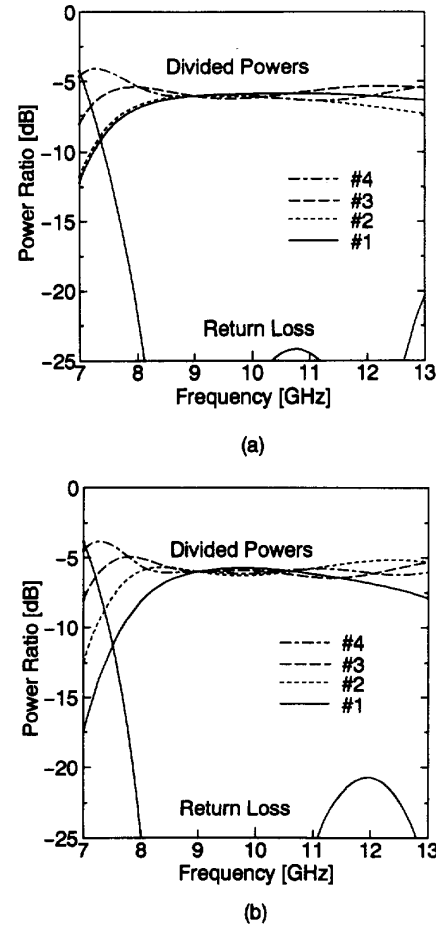
Fig. 4. Frequency characteristics of the four-stage (eight-way) divider. (a) Case when unit #1 is reflectionless (case A). (b) Case when the simple structure is used as unit #1 (case B).
