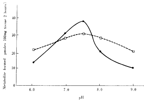
Fig. 5. pH dependence of the formation of testosterone metabolites. Krebs-Ringer-0.1 M phosphate buffer (pH 6.0-8.0) and Krebs-Ringer 0.05 M tris-HCl buffer (pH 8.0-9.0) were used. \bullet — \bullet , Dihydrotestosterone; \square — \square , \triangle -Androstenedione.
