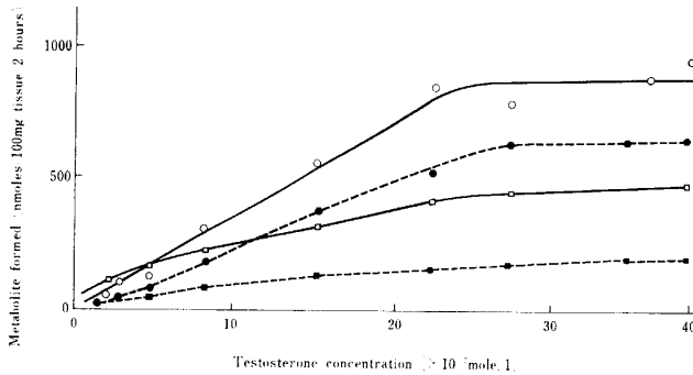
Fig. 4. The rate of formation of testosterone metabolites increased in proportion to the concentration of the substrate. ^{14}\text{C} -Testosterone was incubated with 500 mg of minced skin. \circ — \circ , Dihydrotestosterone; \bullet — \bullet , Androstandiol; \square — \square ; \triangle -Androstenedione; \blacksquare — \blacksquare Androstenedione.
