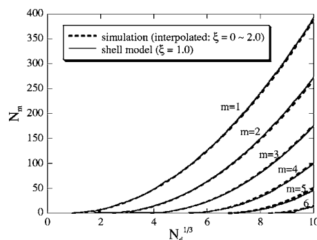
FIG. 8. Populations on shells. Solid lines are values given by the shell model. Dotted lines are results of simulations expressed by an interpolation.
