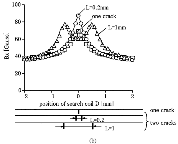
Fig. 11. Changes of (a) |B_z| and (b) |B_x| by search coil position ( C_w = 0.02 mm, C_l = 100 mm).
