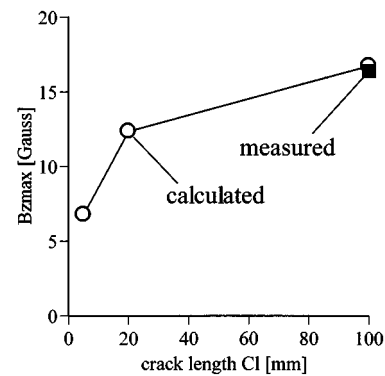
Fig. 7. Effect of crack length Cl on Bz ( Cw = 0.02 \text{ mm} , D = 1 \text{ mm} ).
