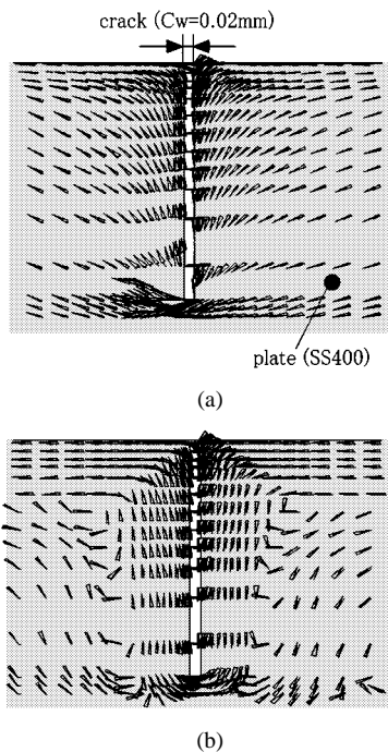
Fig. 5. Comparison of flux distributions at linear and nonlinear analyses ( Cw = 0.02 \text{ mm} , I = 1 \text{ A(rms)} ). (a) Linear analysis ( \mu_s = 3000 , |B|_{\text{max}} = 21.2 \text{ T} ). (b) Nonlinear analysis [(2.25ms/36 steps), |B|_{\text{max}} = 1.69 \text{ T} ].
