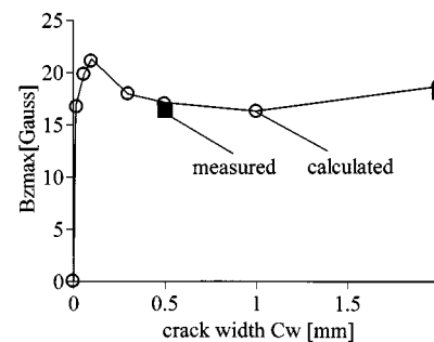
Fig. 8. Effect of crack width Cw on Bz ( Cl = 100 \text{ mm} , D = 1 \text{ mm} ).
