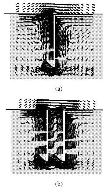
Fig. 9. Flux distribution near one crack and two cracks ( Cw = 0.02 \text{ mm} , Cl = 1 \text{ mm} ). (a) One crack. (b) Two cracks ( L = 0.2 \text{ mm} )
